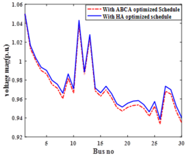
Fig.2. System voltage profile with HA and ABCA optimized schedule
